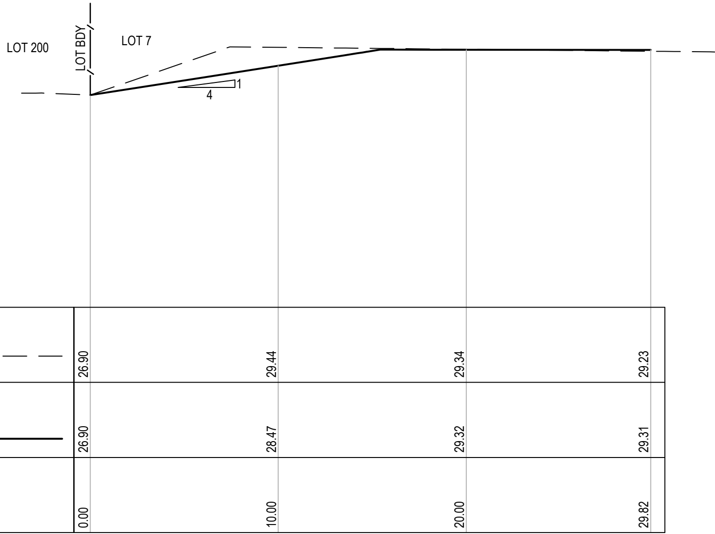
SECTION F HORIZONTAL SCALE 1:1500@A1 VERTICAL SCALE 1:250@A1
