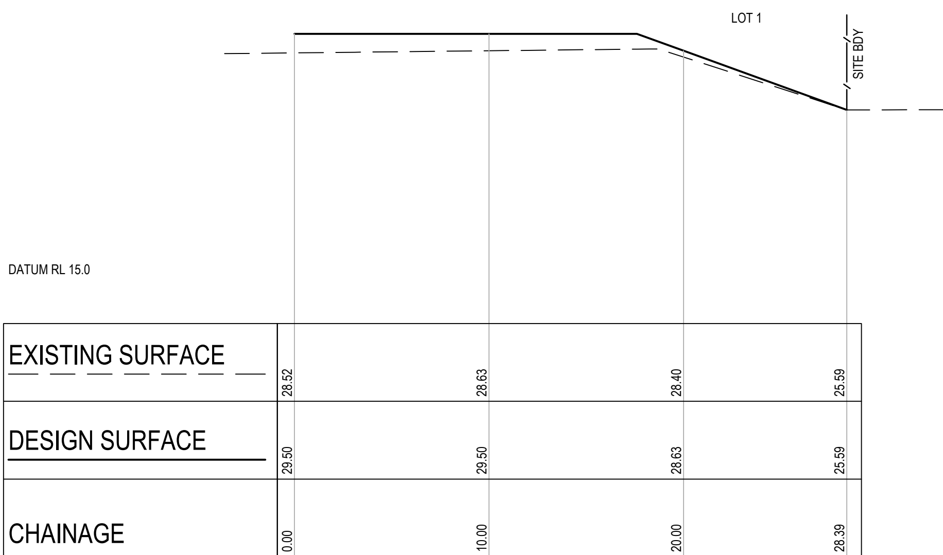
SECTION J HORIZONTAL SCALE 1:1500@A1 VERTICAL SCALE 1:250@A1
