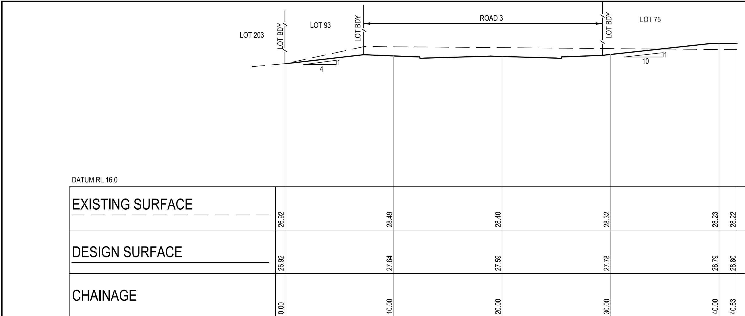
SECTION F HORIZONTAL SCALE 1:1500@A1 VERTICAL SCALE 1:250@A1
