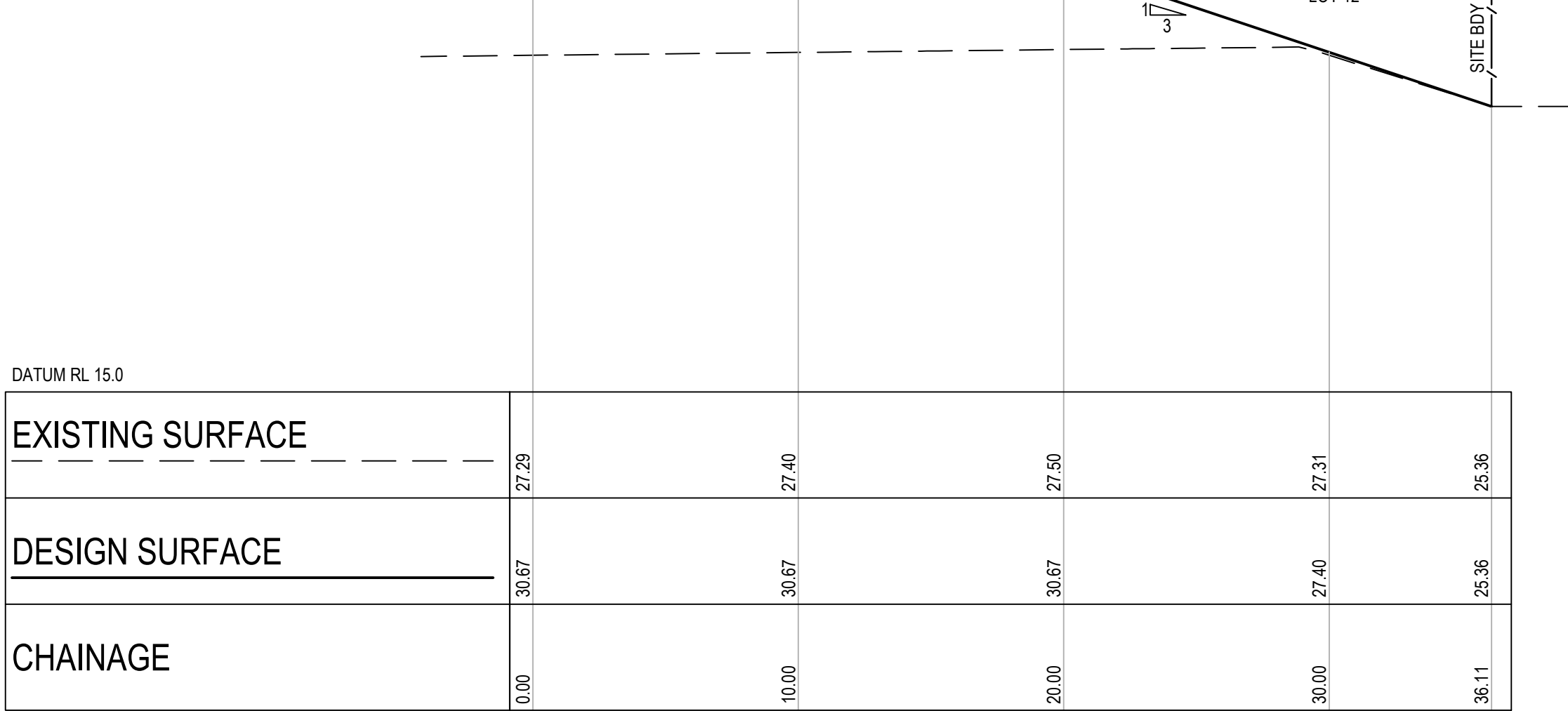
SECTION K HORIZONTAL SCALE 1:1500@A1 VERTICAL SCALE 1:250@A1
