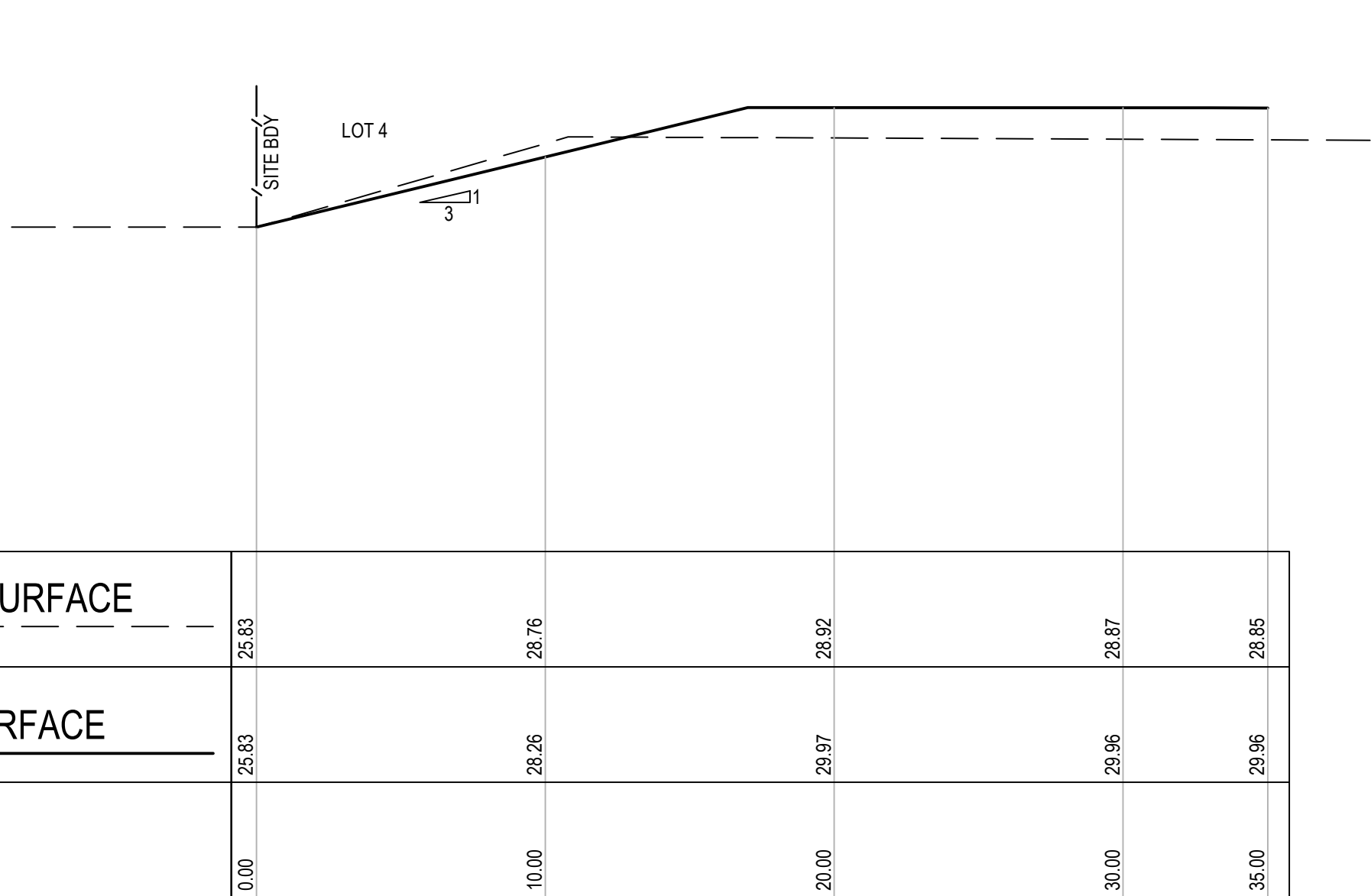
SECTION I HORIZONTAL SCALE 1:1500@A1 VERTICAL SCALE 1:250@A1
