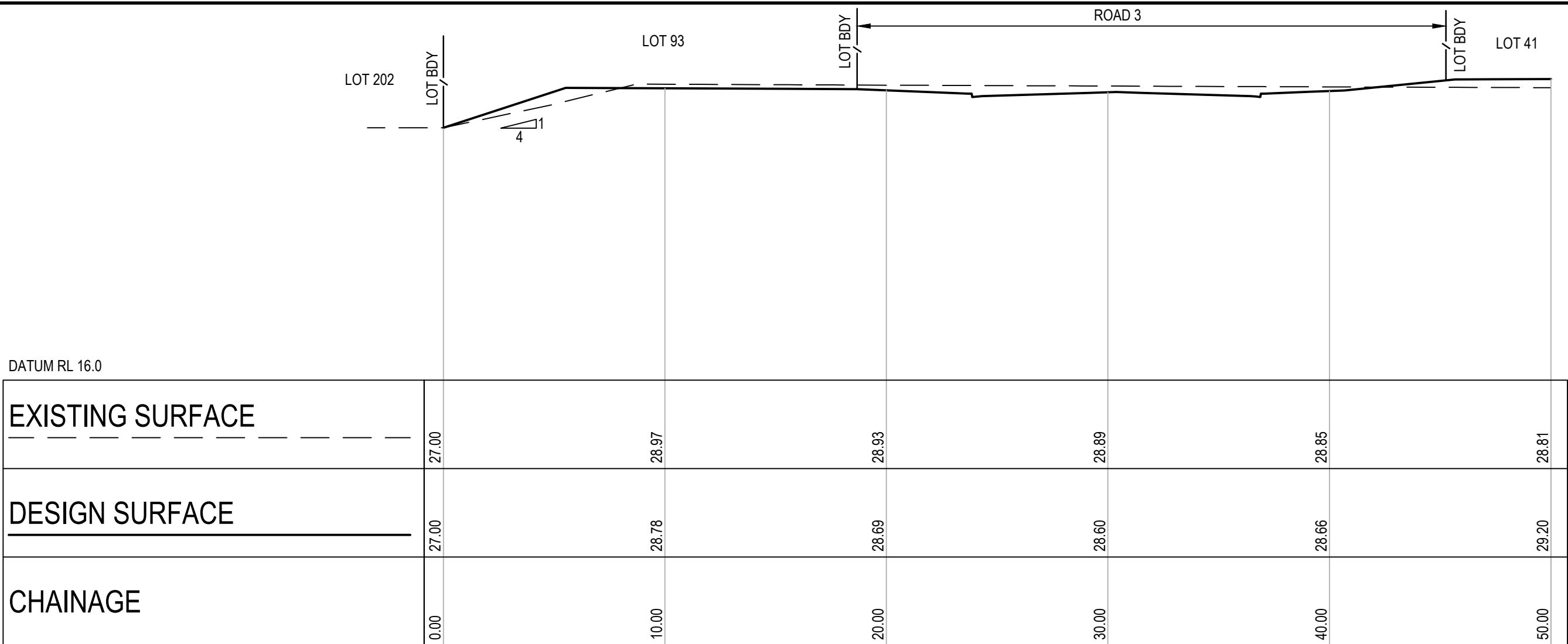
SECTION G HORIZONTAL SCALE 1:1500@A1 VERTICAL SCALE 1:250@A1
